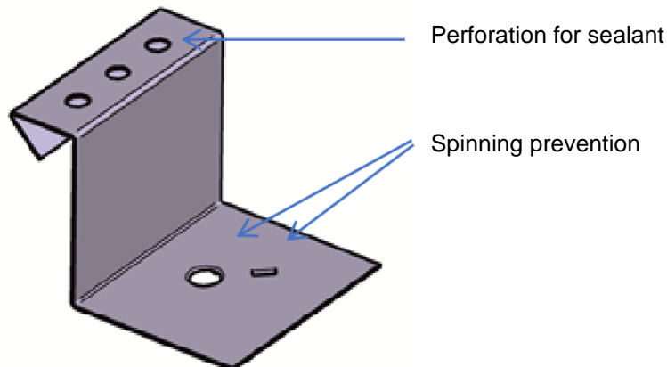
1. Perforated cleat
