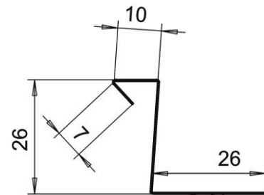
2. Dimensional drawing of the cleat
