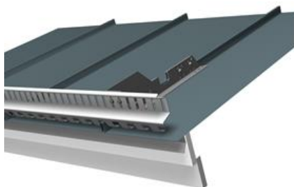
1. VARMA 120 for standing seam roofing (mechanical lock)
